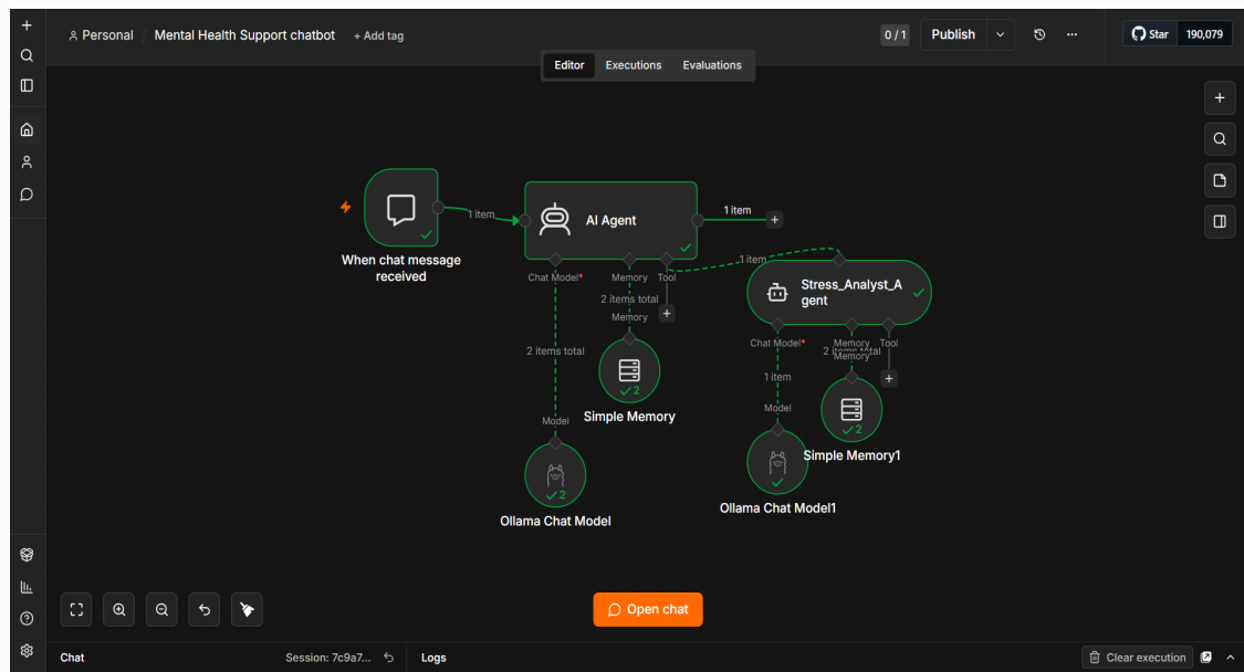
Figure 3.5: Visual Graph Assembly Canvas interface within n8n Workspace environments.
